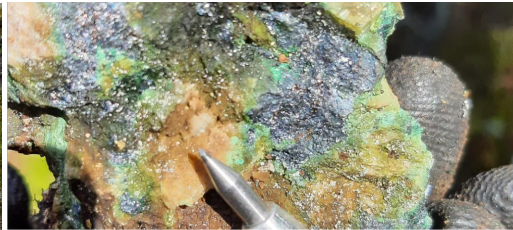
(b) #C879209 – carbonate and bornite, malachite vein 25.60 % Cu, 4.90 g/t Au, 162.0 g/t Ag
